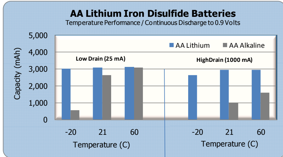
(fig. 4) Temperature Effect on Performance Versus Alkaline
