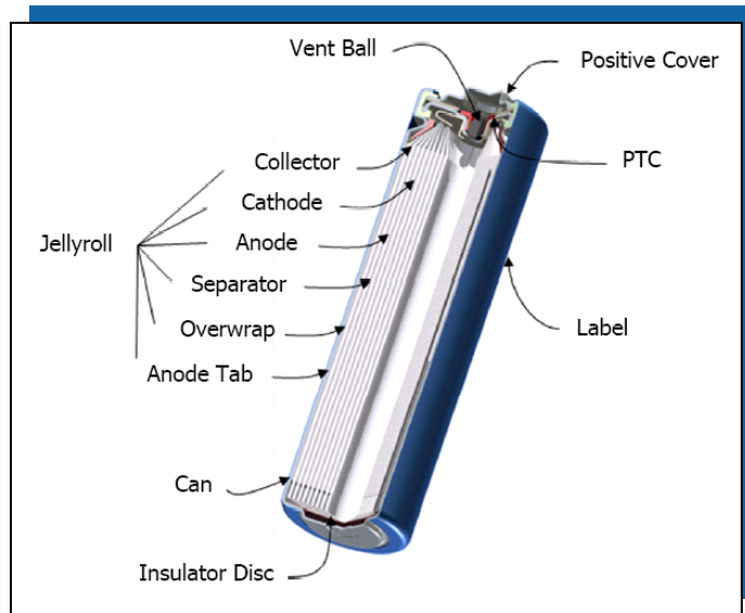
(fig. 1) Typical cylindrical lithium iron disulfide battery
