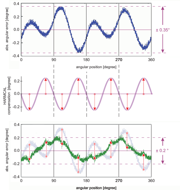
Figure 8: Harmonic calibration
