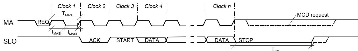
Figure 2: Timing diagram in BiSS C protocol.
