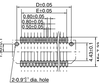
Recommended PC board pattern (TOP VIEW)
