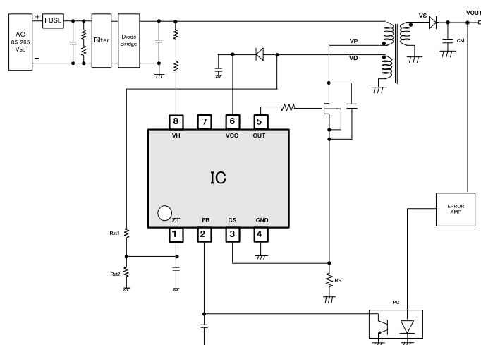
Fig 1. Application Circuit
