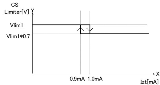
Fig-20 Izt Current vs Switched CS Voltage Characteristics
