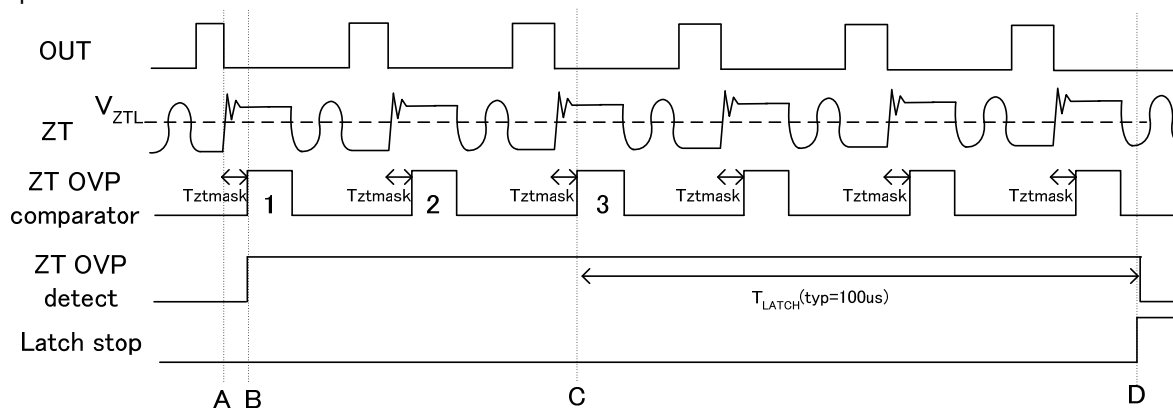
Fig-24 ZTOVP and Latch Blanking Function
