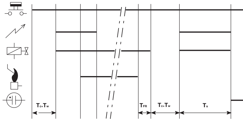
Fig. 14. Functional diagram S4565AM, BM, PM, QM
