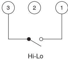
Fig. 7. Connection S4565BM,DM, QM, TM with Hi-Lo
