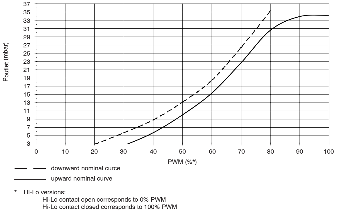
Fig. 2. Nominal graph modulating performance at 37 mbar inlet pressure, Ø 2.8 mm outlet restriction
