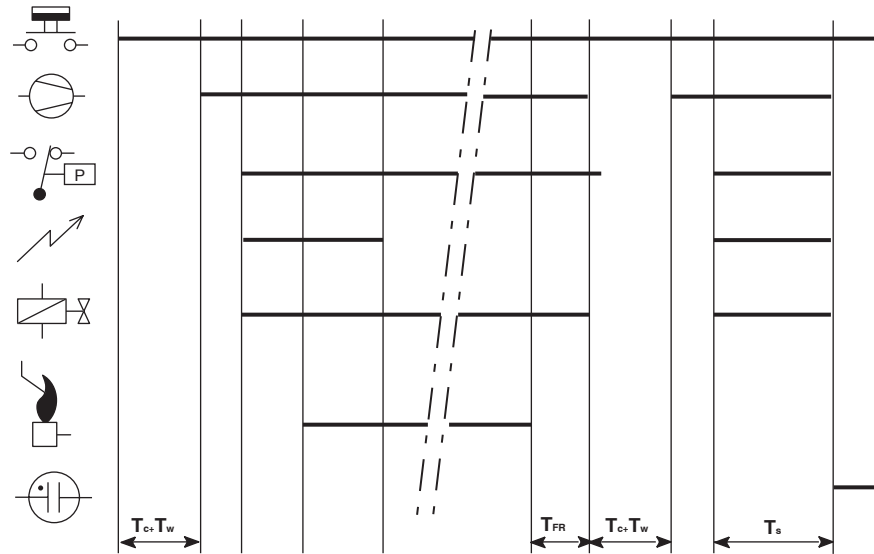
Fig. 15. Functional diagram S4565CM, DM, RM, TM
