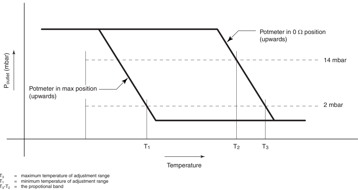
Fig. 3. Nominal graph modulating performance in case of CVI-m with NTC and proportional control
