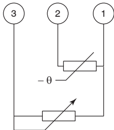
Fig. 9. Connection S4565AM, BM, CM, DM, PM, QM, RM, TM with NTC sensor and external potentiometer for temperature setpoint
