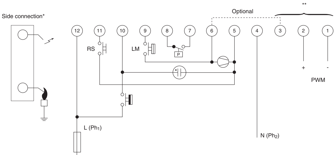
Fig. 4. Connection diagram S4565AM, BM, PM, QM
