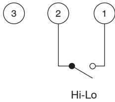
Fig. 6. Connection S4565AM, CM, PM, RM with Hi-Lo
