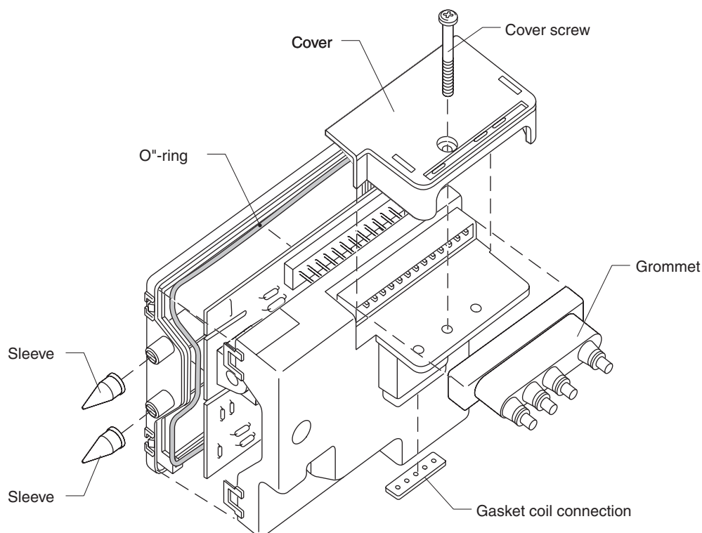
Fig. 19. S4565xM exploded view IP 44 enclosure
