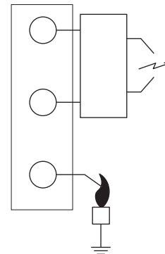
Fig. 11. Side connection for combined ignition and flame sensing
