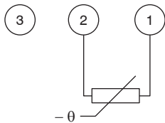
Fig. 8. Connection S4565AM, BM, CM, DM, PM, QM, RM, TM with NTC sensor
