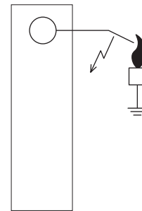
Fig. 11. Side connection for combined ignition and flame sensing
