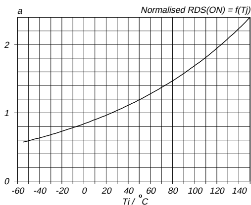
Fig. 9. Normalised drain-source on-state resistance. a = R_{DS(ON)}/R_{DS(ON)25^\circ\text{C}} = f(T_j) ; I_D = 3 \text{ A} ; V_{GS} = 10 \text{ V}
