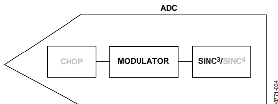
Figure 32. Sinc 3 Filter (Chop Disabled)
