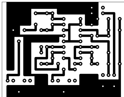
Copper Side 2.2" x 1.7"
