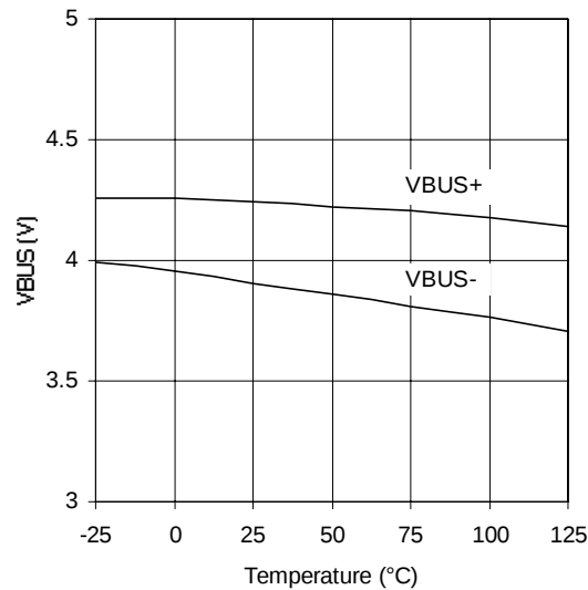
Graph 12: VBUS+, VBUS- vs TEMP
