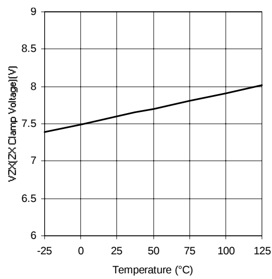
Graph 10: VZX (ZX Clamp Voltage) vs TEMP
