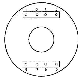
DEFLECTION YOKE
