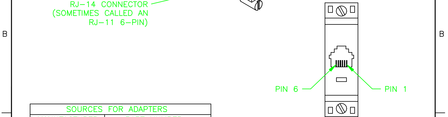
FRONT VIEW FOR RJ-14 CONNECTOR
