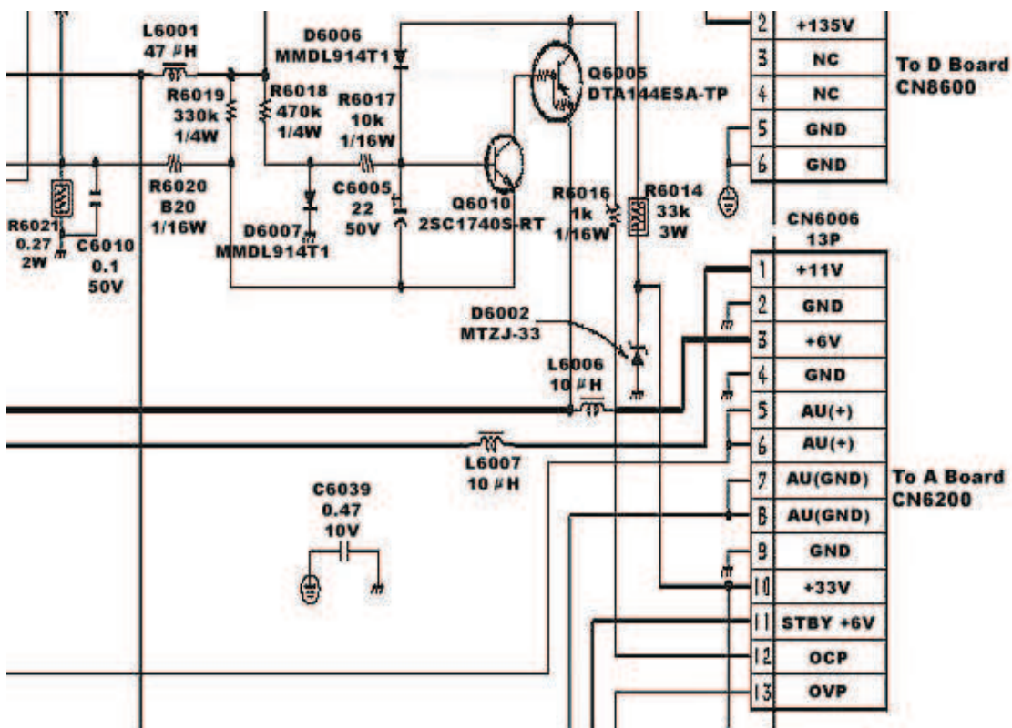
Figure 2.6 Overcurrent Protection
