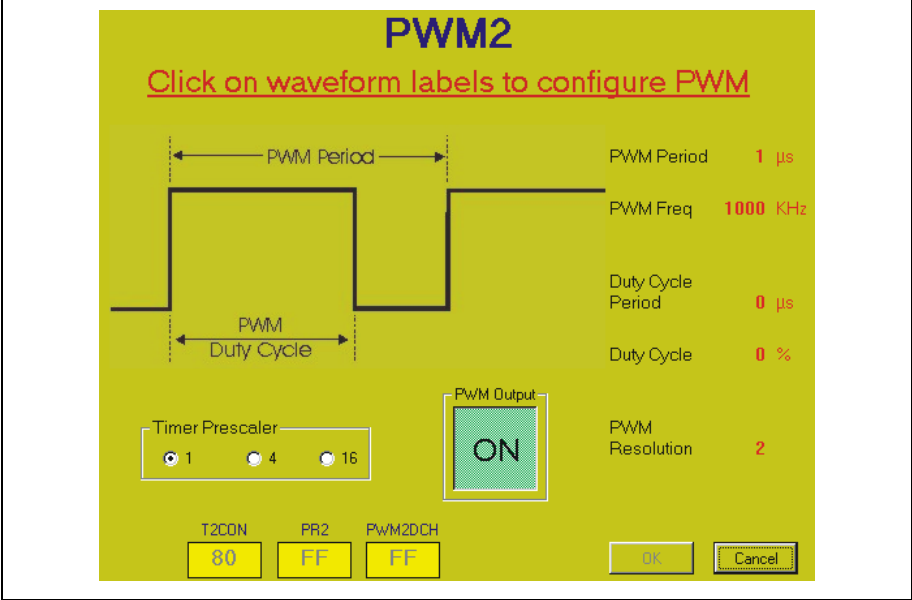
FIGURE 4.5: PWM MODULES
