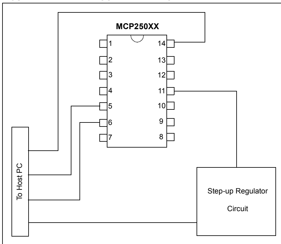
FIGURE 4.1: DEVICE PROGRAMMER DIAGRAM
