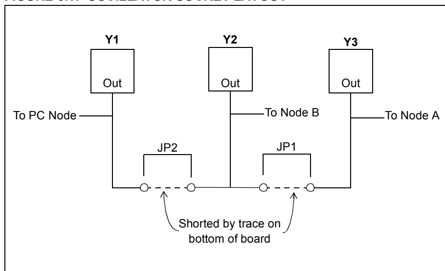
FIGURE 5.1: OSCILLATOR SOCKET LAYOUT
