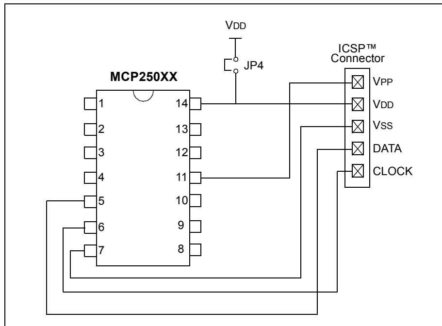
FIGURE 4.8: PROGRAMMING VIA THE ICSP™ CONNECTOR
