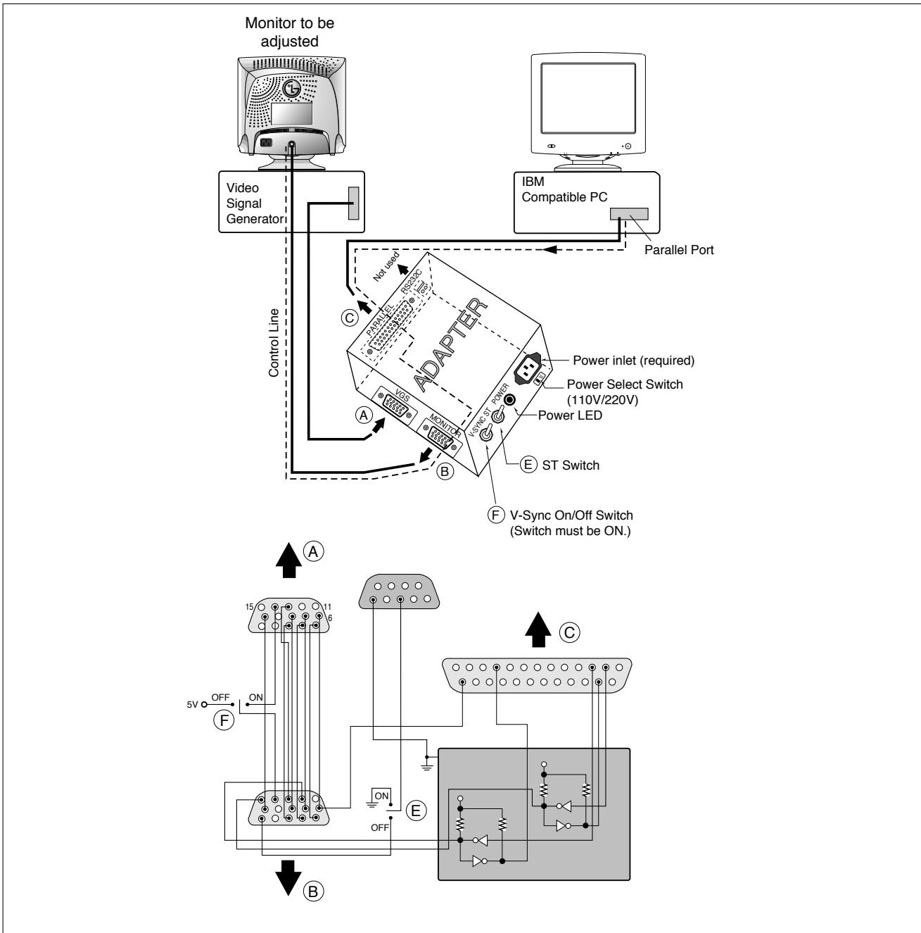
Figure 1. Cable Connection
