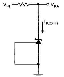
TEST CIRCUIT 3
