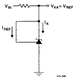
TEST CIRCUIT 1
