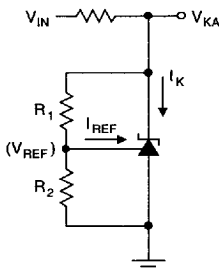
TEST CIRCUIT 2
