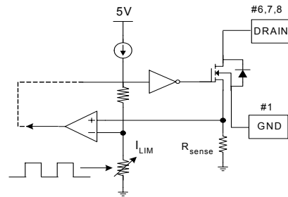
Figure 7. Soft Start Function
