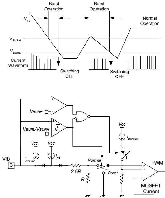
Figure 8. Burst Operation Function
