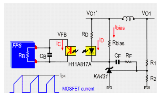
Figure 14. Typical Feedback Network of FPS
