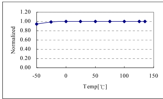
Frequency Modulation (ΔFMOD) vs. Ta
