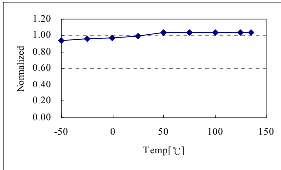
Operating Frequency (Fosc) vs. Ta
