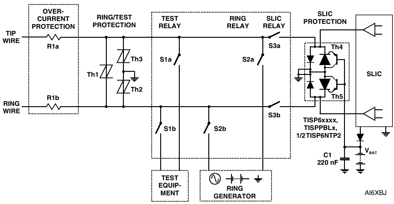
Figure 17. Line Card Ring/Test Protection
