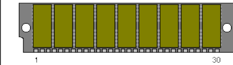
30 pin SIMM connector
