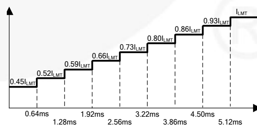
Figure 19. Current Limit Variation During Soft-Start
