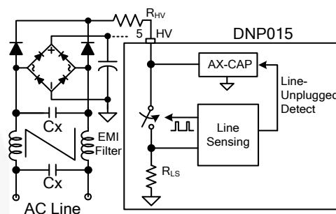
Figure 22. AX-CAP® Circuit
