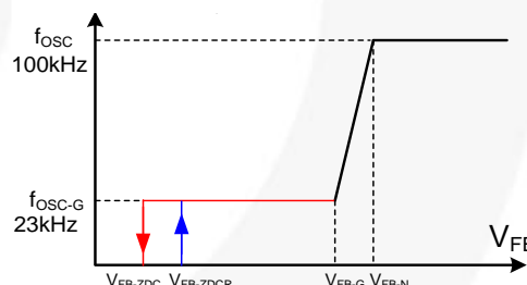
Figure 23. PWM Frequency
