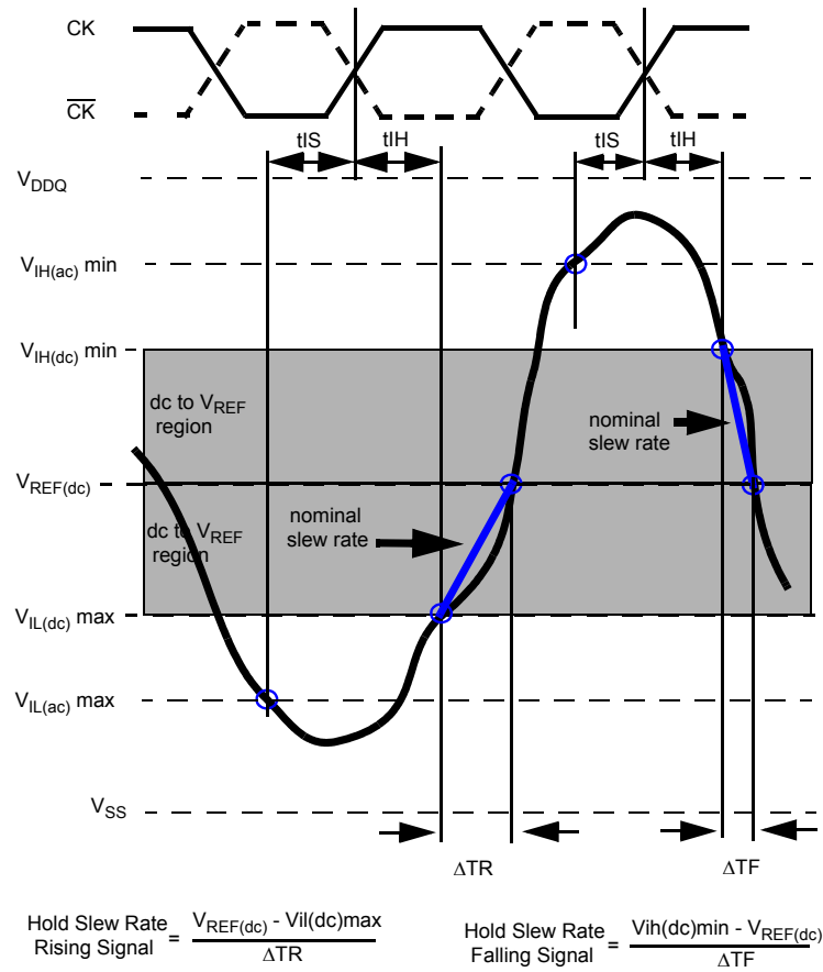
Figure 15 - Illustration of nominal slew rate for tIH
